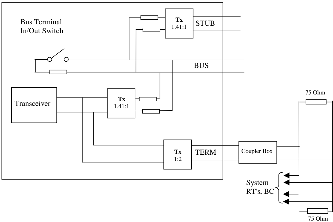
Figure 13-6 Monitoring of an External System
