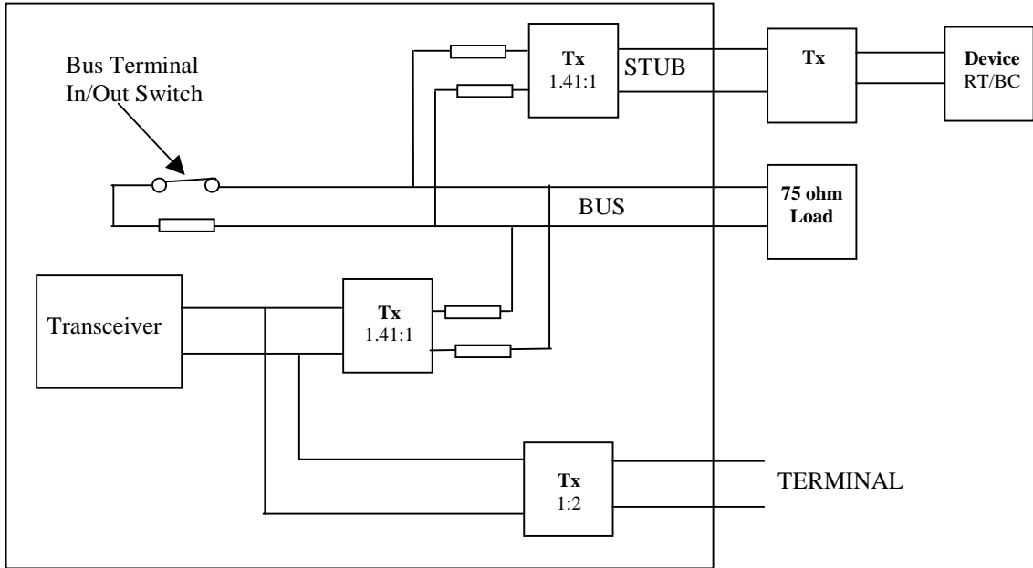
Figure 13-2 Bench testing Transformer Coupled Device (when no external 1553 bus is available) Bus Terminal Switch IN
