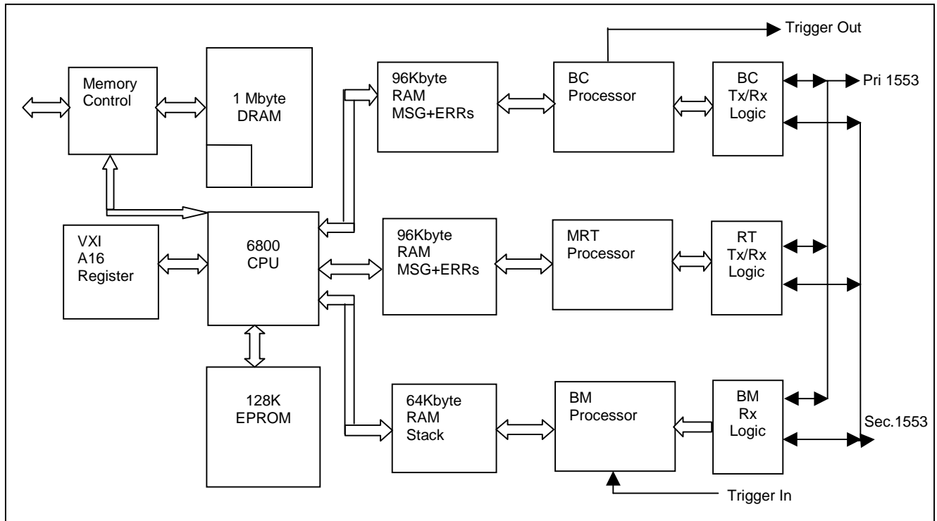
Figure 3-1 SURETEST 2704 Block Diagram
