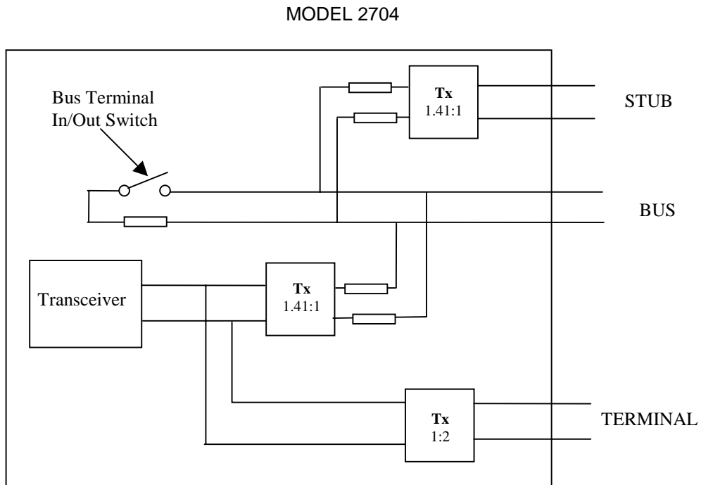
Figure 13-1 1553 Bus Interface
