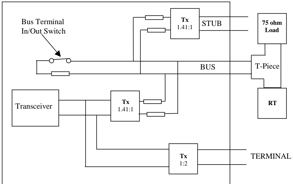
Figure 13-3 Bench testing Direct Coupled Stub on 1553 device Bus Terminal Switch IN
