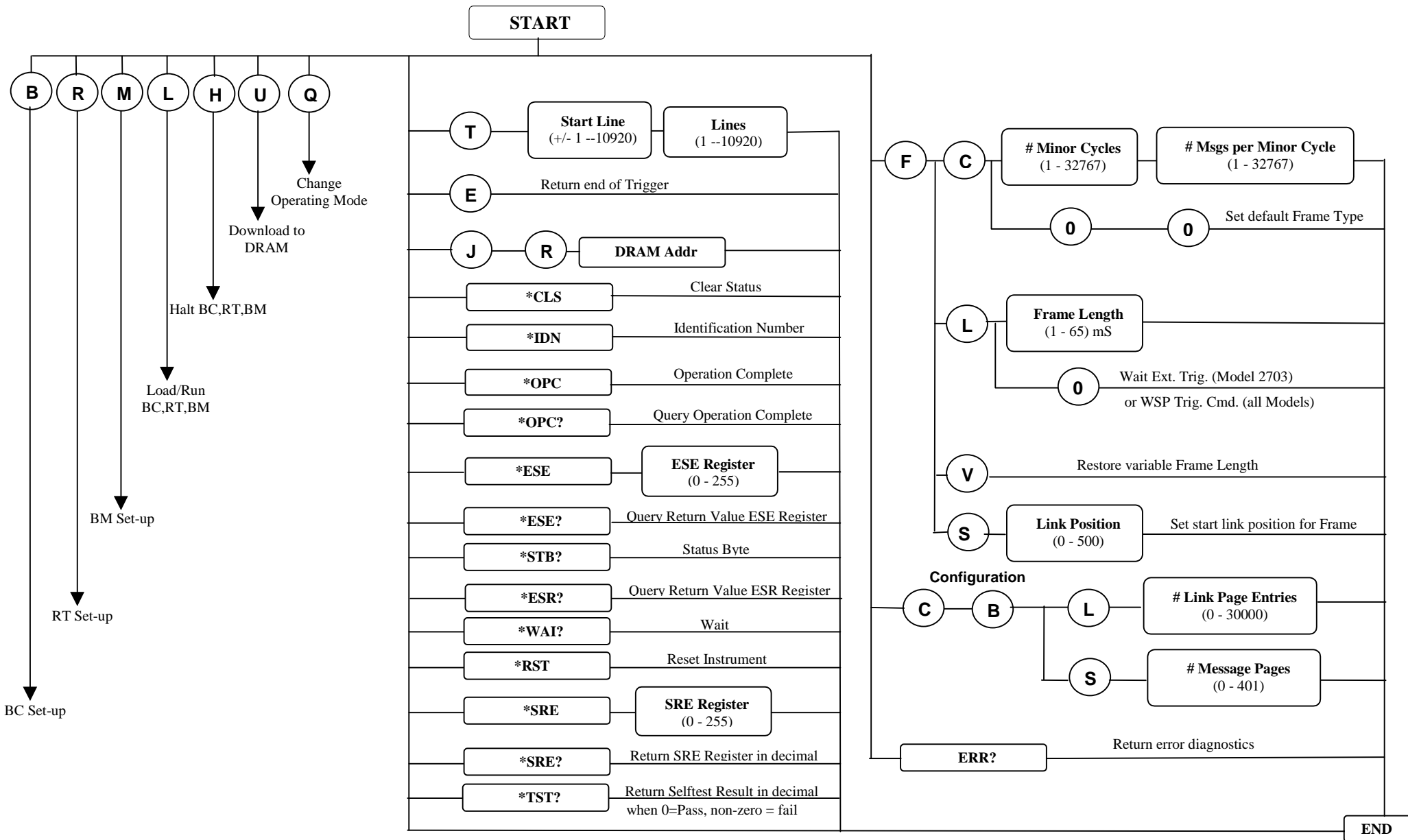
Figure 3-4 Top Level Syntax Diagram
